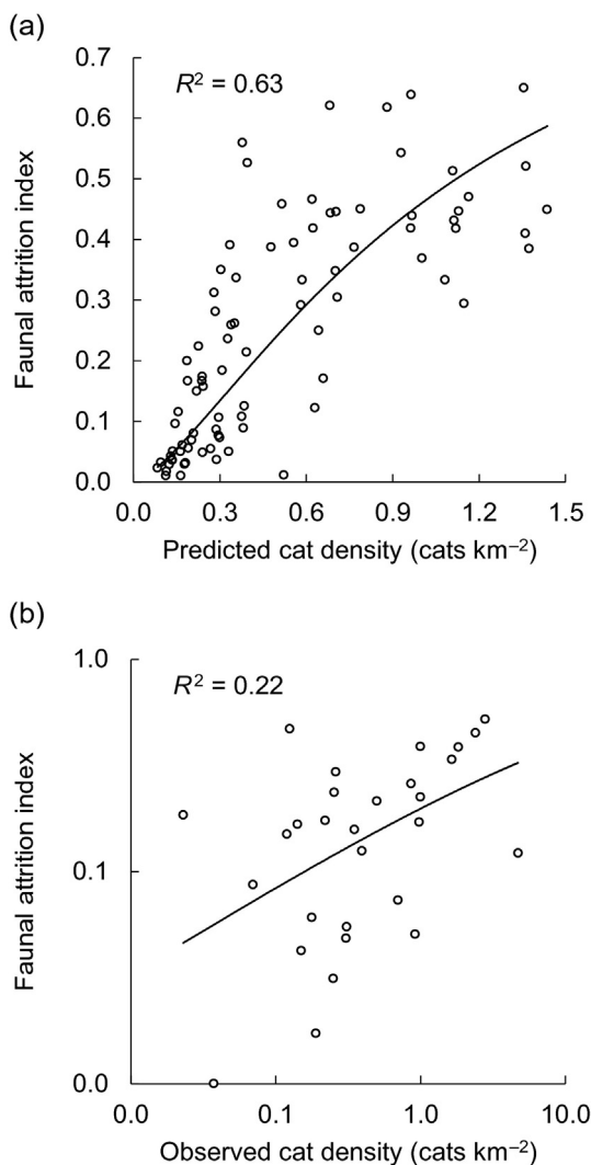
Fig. 6. Relationships between the regional attrition of native, non-flying mammals (Burbidge et al., 2008) and the (a) predicted and (b) observed feral cat densities in each bioregion following a wet period. The regression lines are linear regressions of the form: Faunal attrition index (FAI) ~ density, with FAI logit-transformed and density log-transformed prior to analysis.
